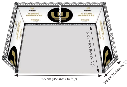
Model 775 / UCT15BM775 Truss U-Shape 4 x 6
