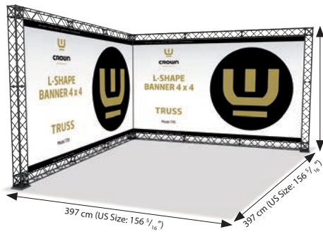
Model 770 / UCT15BM770 Truss L-Shape 4 x 4
