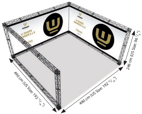
Model 773 / UCT15BM773 Truss U-Shape 5 x 5
